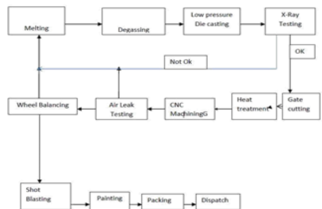
Figure 1.1. Process flow diagram for manufacturing of Al alloy wheel.
