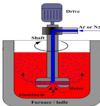
Figure Rotary degassing method
